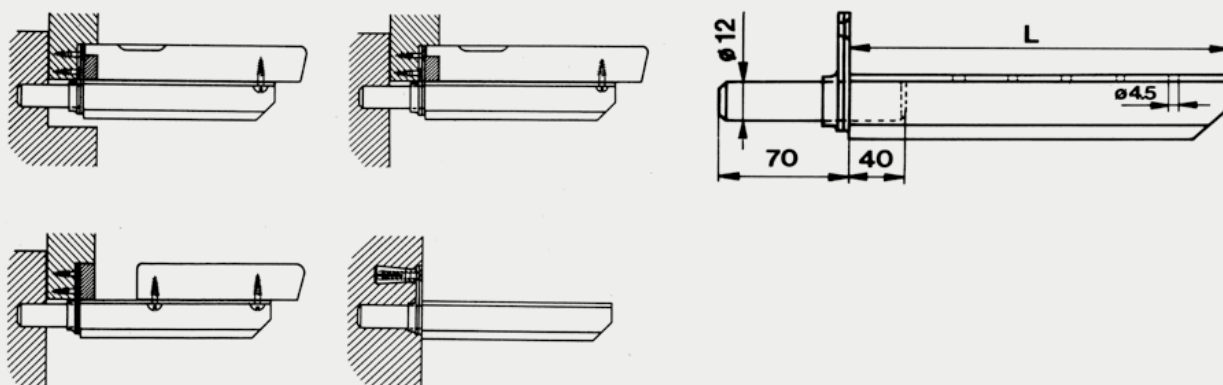
Installation exemples
